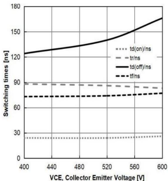
Figure 15: Typical Switching Times vs. VCE ( T_J=25^{\circ}\text{C} , V_{GE}=15/0\text{V} , I_C=60\text{A} )
