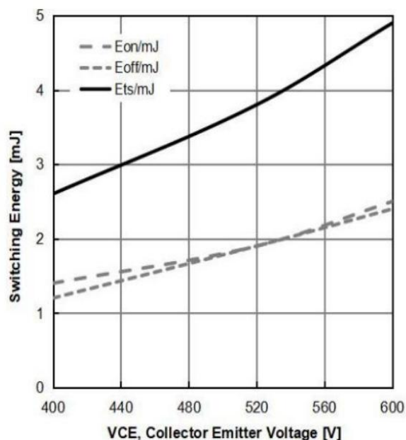
Figure 16: Typical Switching Energy vs. VCE ( T_J=25^{\circ}\text{C} , V_{GE}=15/0\text{V} , I_C=60\text{A} )
