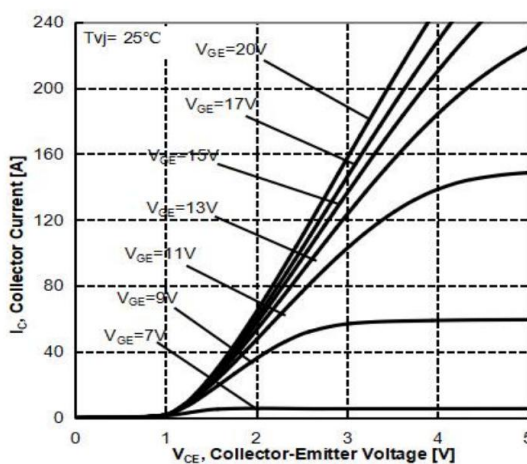
Figure 5: Output Characteristics
