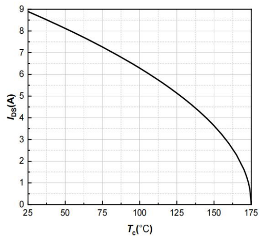
Figure 18. Continuous Drain Current Derating vs. Case Temperature
