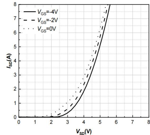
Figure 10. Body Diode Characteristic T_J=170^{\circ}\text{C}
