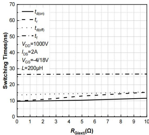
Figure 23. Switching Times vs. R_{G(ext)}
