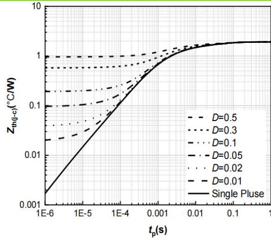
Figure 20. Transient Thermal Impedance
