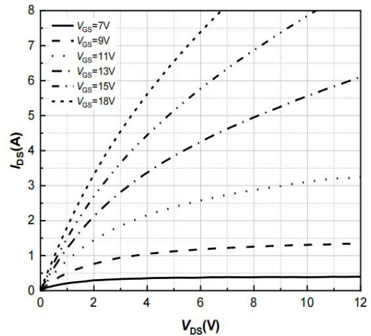
Figure 2. Output Characteristics
