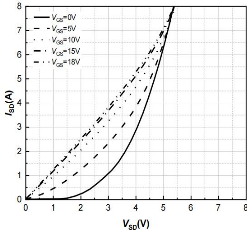
Figure 15. 3rd Quadrant Characteristic T_j=175^{\circ}\text{C}
