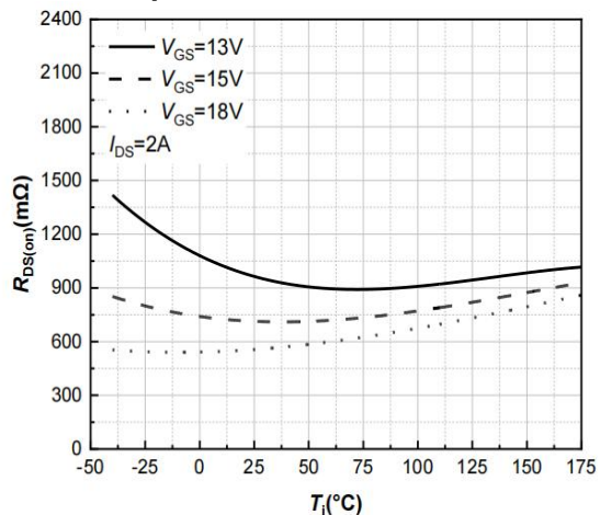
Figure 6. On-Resistance vs. Temperature For Various Gate Voltage
