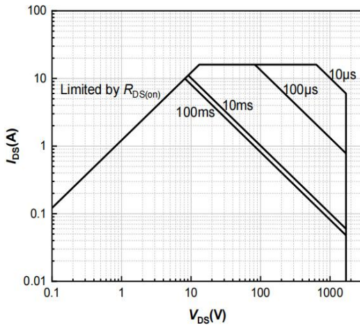
Figure 24. Safe Operating Area
