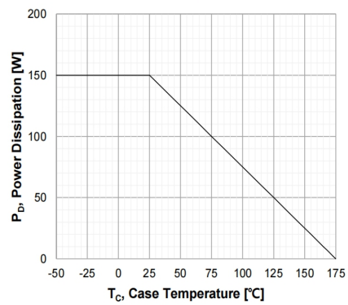
Figure 16. Maximum Power Dissipation Derating vs. Case Temperature
