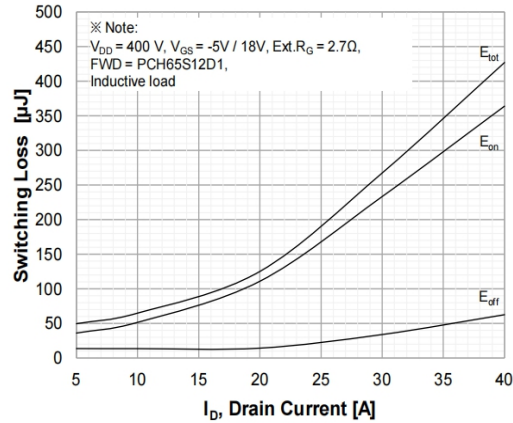
Figure 17. Typ. Switching Losses vs. Drain Current
