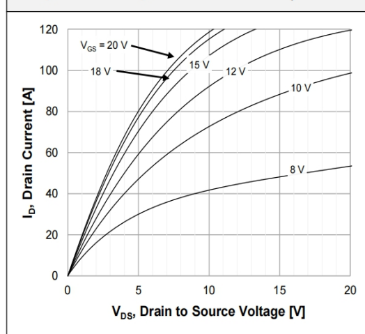
Figure 4. On-Region Characteristics T_J = 175^\circ\text{C}
