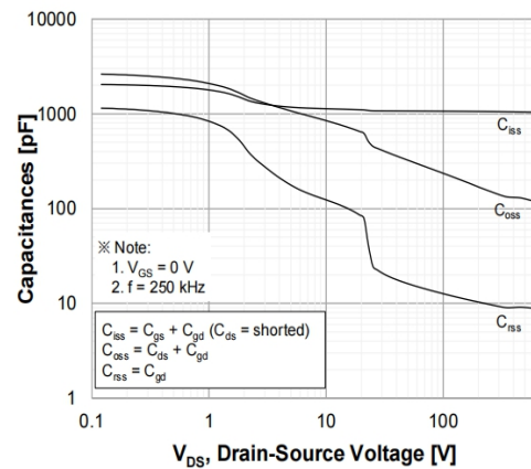
Figure 14. Capacitance Characteristics
