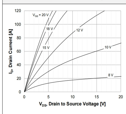
Figure 2. On-Region Characteristics T_J = 25^\circ\text{C}
