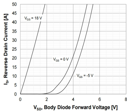
Figure 8. Diode Forward Voltage Characteristics vs. Source-Drain Current T_J = 25^{\circ}\text{C}
