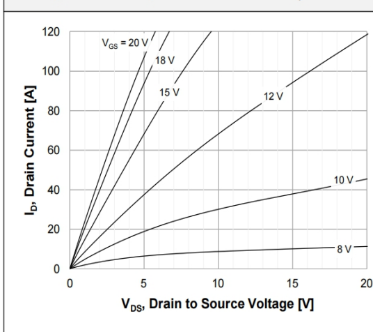
Figure 1. On-Region Characteristics T_J = -40^\circ\text{C}
