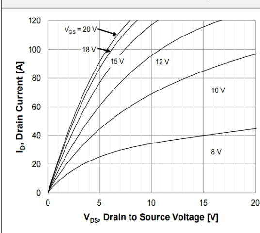
Figure 3. On-Region Characteristics T_J = 125^\circ\text{C}
