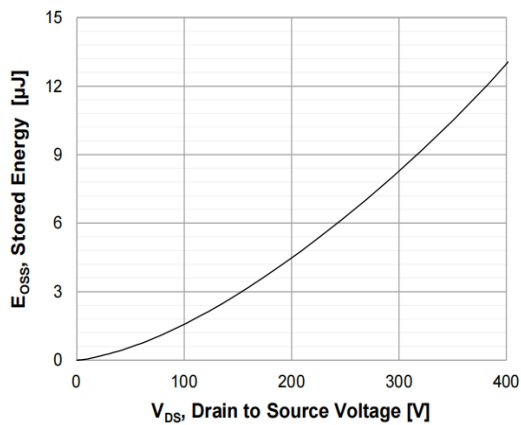
Figure 13. Stored Energy in Output Capacitance
