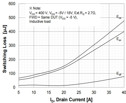
Figure 19. Typ. Switching Losses vs. Drain Current
