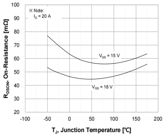
Figure 5. On-Resistance Characteristics vs. Temperature
