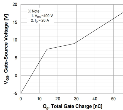
Figure 12. Gate Charge Characteristics
