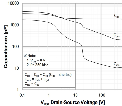
Figure 14. Capacitance Characteristics
