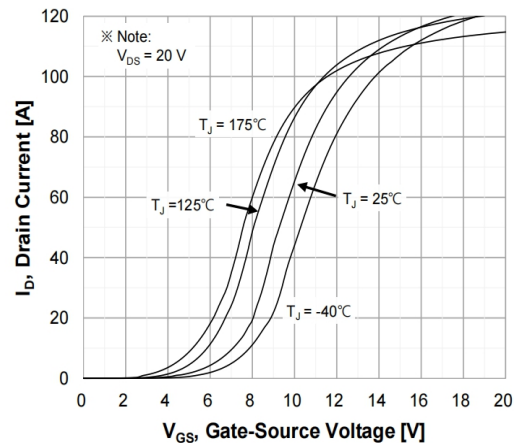
Figure 6. Transfer Characteristics
