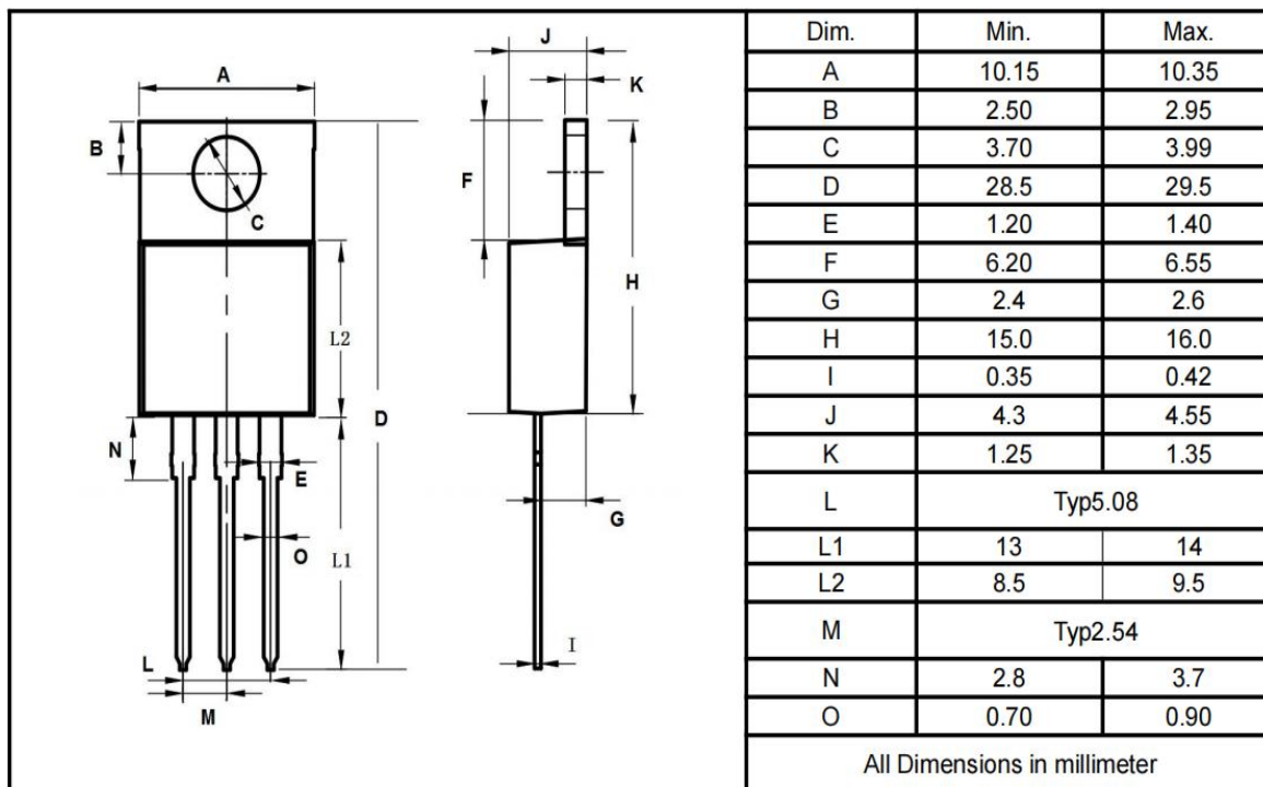
TO-220AB
