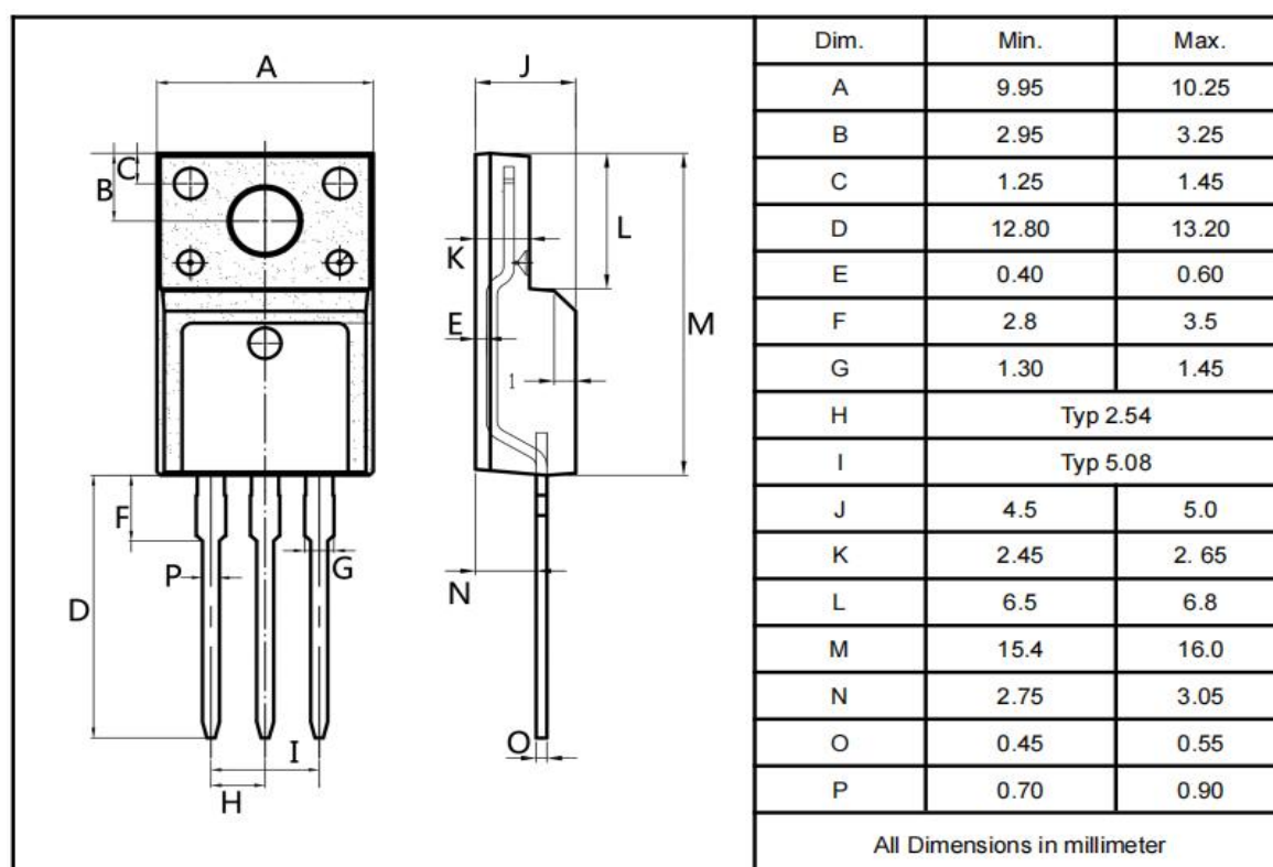
TO-220F
