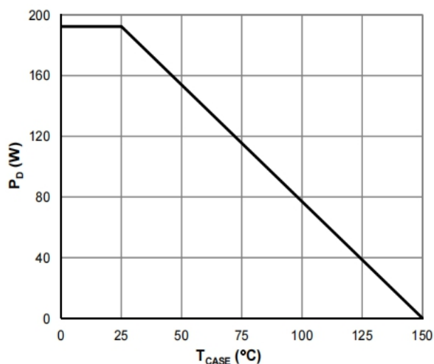
Figure 10: Power De-rating
