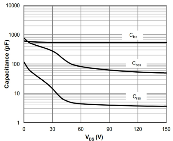
Figure 6: Capacitance Characteristics
