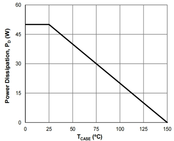
Figure 8: Power De-rating
