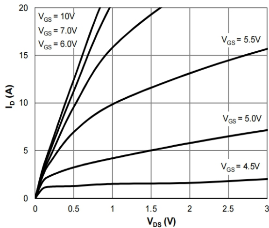
Figure 1: Saturation Characteristics
