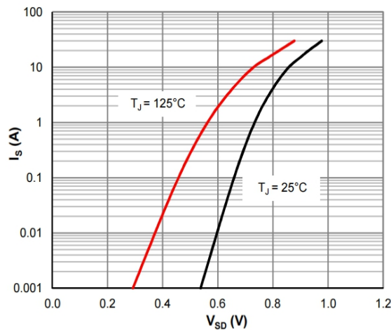
Figure 5: Body-Diode Characteristics
