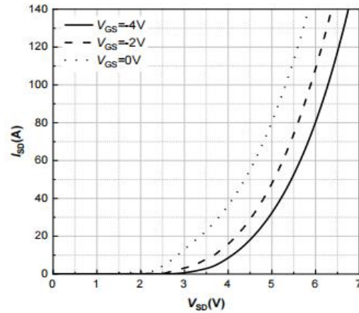
Figure 8. Body Diode Characteristic
