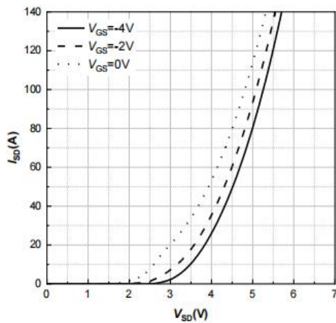
Figure 9. Body Diode Characteristic T_J = 25^\circ\text{C}
