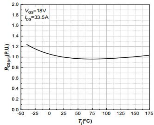
Figure 4. Normalized On-Resistance vs. Temperature
