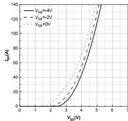
Figure 10. Body Diode Characteristic T_J = 175^\circ\text{C}
