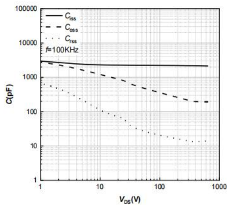
Figure 17. Capacitances vs. Drain-Source
