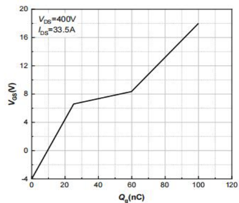
Figure 12. Gate Charge Characteristics
