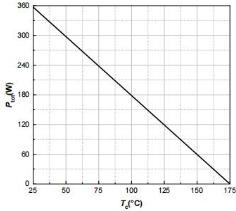
Figure 19. Maximum Power Dissipation Derating vs. Case Temperature
