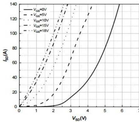
Figure 13. 3rd Quadrant Characteristic T_j = -40^\circ\text{C}
