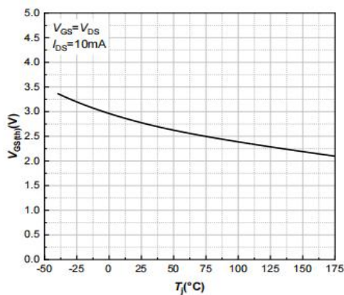
Figure 11. Threshold Voltage vs. Temperature
