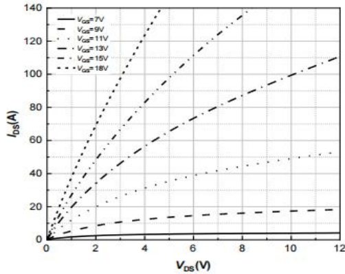
Figure 1. Output Characteristics T_j = -40^\circ\text{C}
