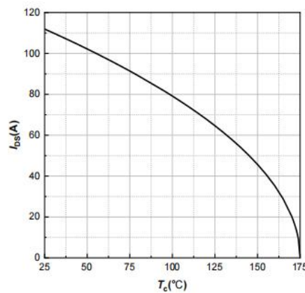
Figure 18. Continuous Drain Current Derating vs. Case Temperature
