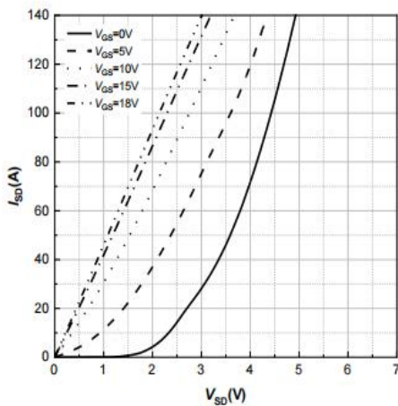
Figure 15. 3rd Quadrant Characteristic T_j = 175^\circ\text{C}
