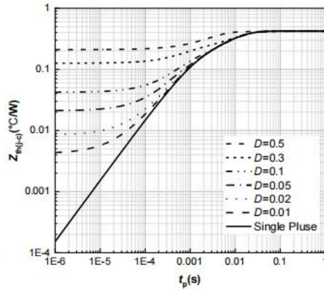
Figure 20. Transient Thermal Impedance
