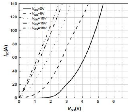
Figure 14. 3rd Quadrant Characteristic T_j = 25^\circ\text{C}
