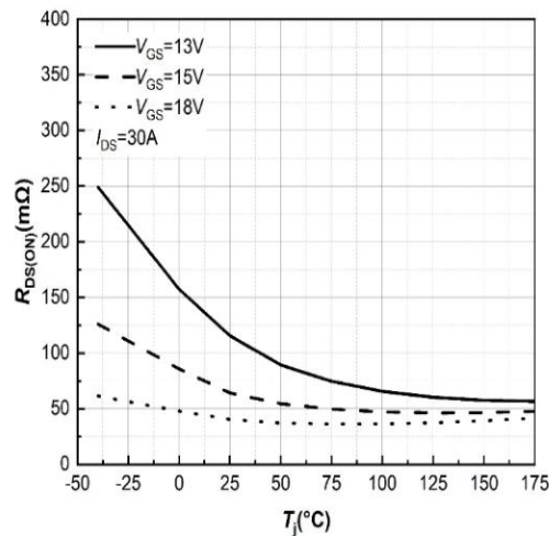
Figure 6. On-Resistance vs. Temperature For Various Gate Voltage
