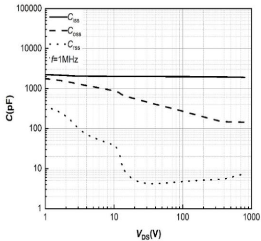
Figure 17. Capacitances vs. Drain-Source
