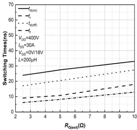
Figure 23. Clamped Inductive Switching Times vs. R_{G(\text{ext})} T_j=25^{\circ}\text{C}
