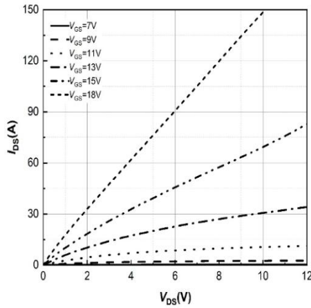
Figure 1. Output Characteristics T_j = -40^\circ\text{C}
