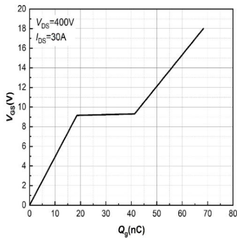
Figure 12. Gate Charge Characteristics
