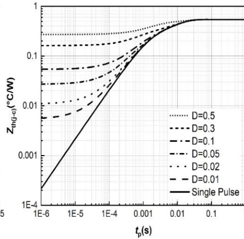
Figure 20. Transient Thermal Impedance
