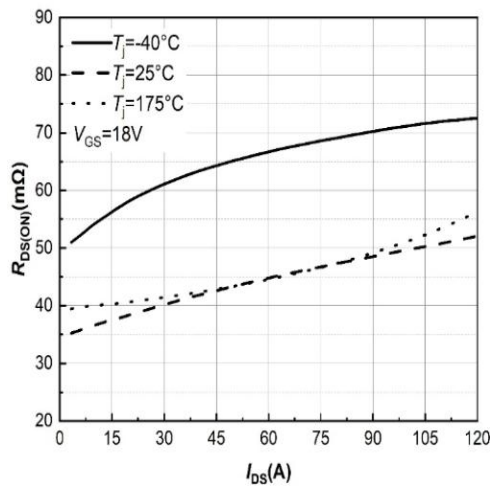
Figure 5. On-Resistance vs. Drain Current For Various Temperatures
