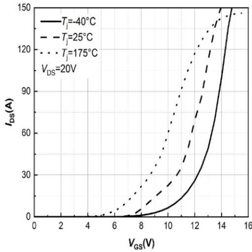
Figure 7. Transfer Characteristic for Various Junction Temperatures
