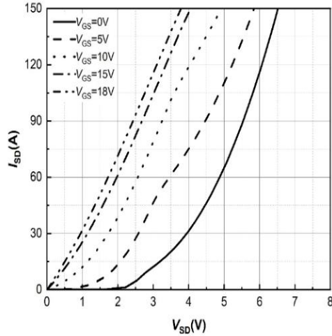
Figure 14. 3rd Quadrant Characteristic T_j = 25^\circ\text{C}
