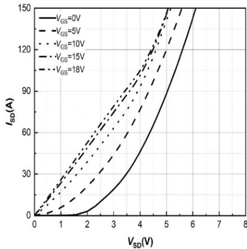
Figure 15. 3rd Quadrant Characteristic T_j = 175^\circ\text{C}
