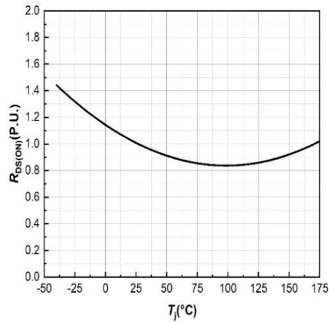
Figure 4. Normalized On-Resistance vs. Temperature
