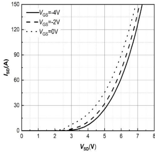
Figure 8. Body Diode Characteristic T_J = -40^\circ\text{C}
