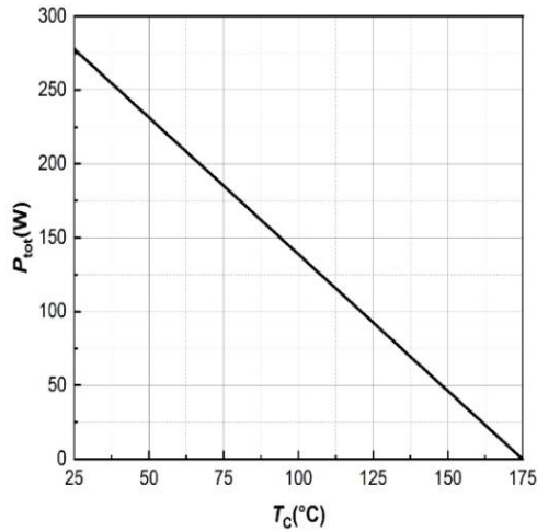
Figure 19. Maximum Power Dissipation Derating vs. Case Temperature
