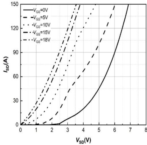
Figure 13. 3rd Quadrant Characteristic T_j = -40^\circ\text{C}
