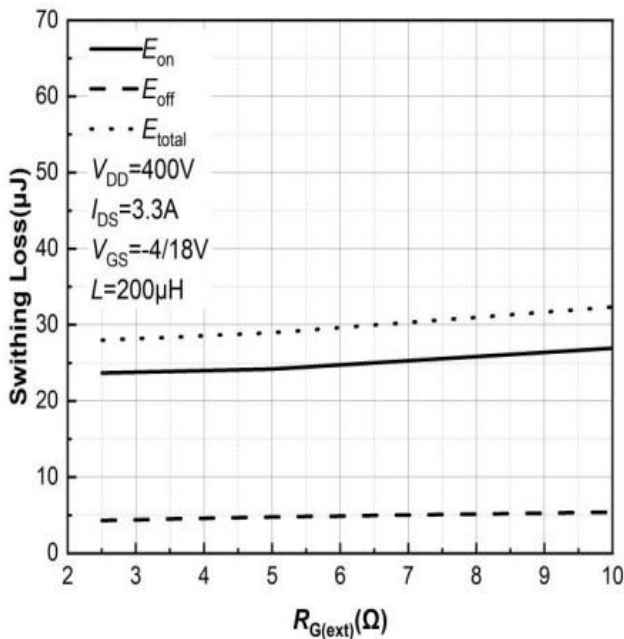
Figure 23. Clamped Inductive Switching Energy vs. R_{G(ext)} T_j = 25^\circ\text{C}
