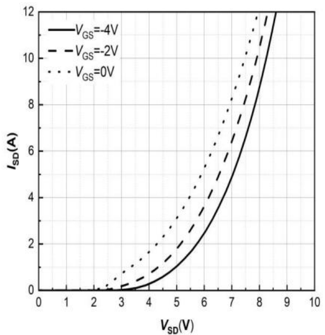
Figure 8. Body Diode Characteristic T_J = -40^\circ C
